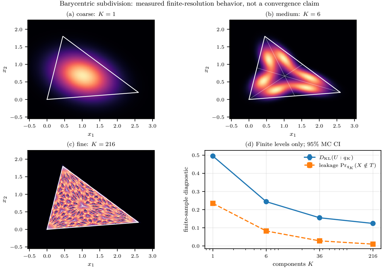
FIGURE 3. Four finite barycentric-subdivision levels show decreasing sampled forward-KL and leakage diagnostics at each displayed level; they do not establish general monotonicity or asymptotic convergence.
