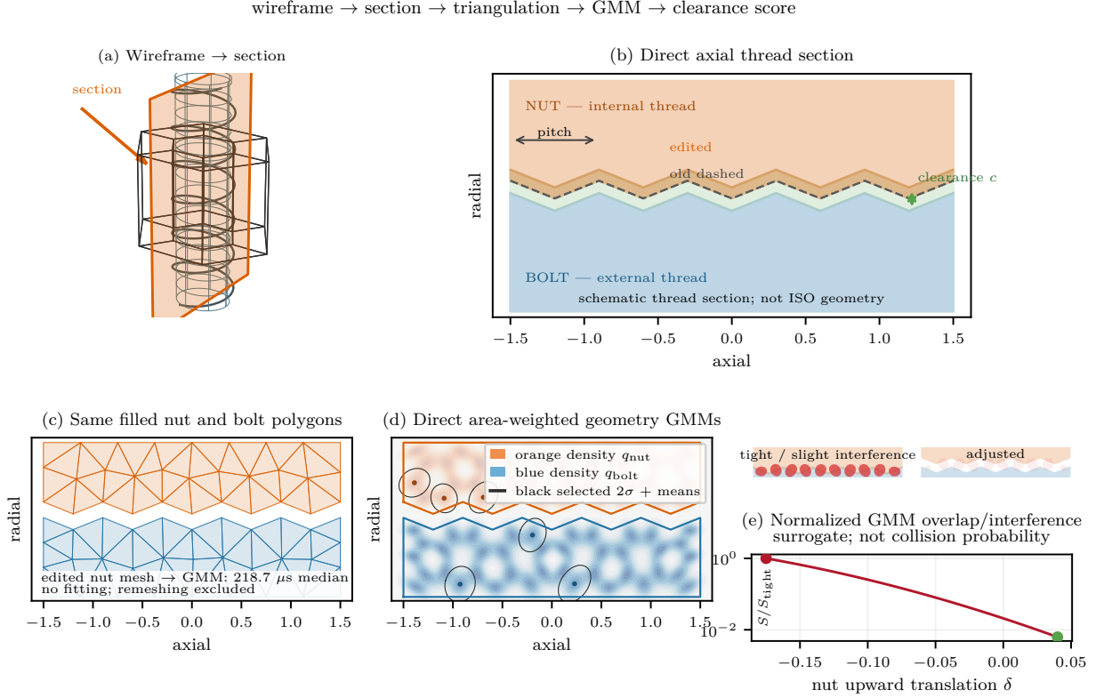
FIGURE 6. A schematic wireframe is sectioned; the same bounded full-dimensional nut and bolt material polygons are directly triangulated and converted to area-weighted geometry GMs. Nut-clearance translations update component means and allow analytic overlap rescoring. Normalized overlap/interference is a soft surrogate, not a collision probability; this is not an ISO, contact, or certification analysis.
