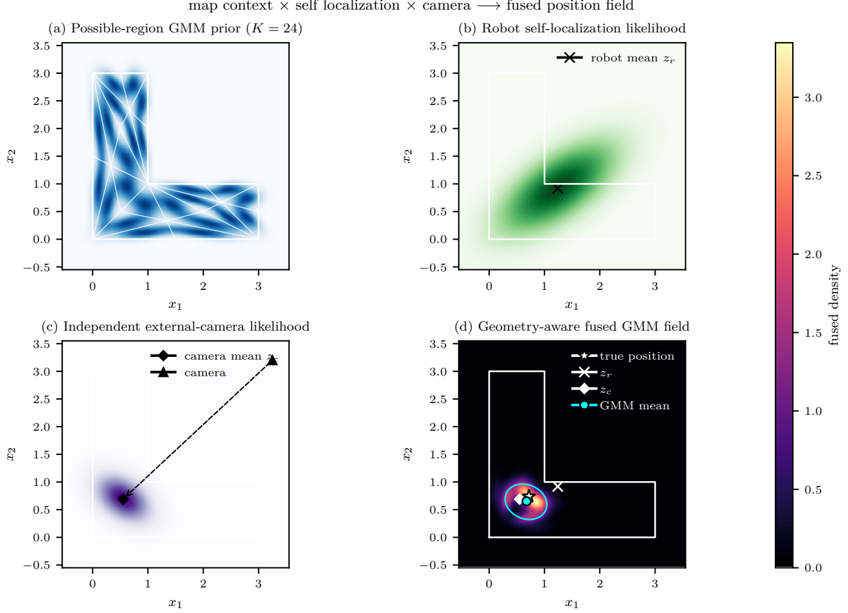
FIGURE 5. A map prior times conditionally independent robot and camera Gaussian likelihoods gives a sequential closed-form update. The contour is a finite-grid constrained reference; no validity is claimed under unknown sensor correlation.
