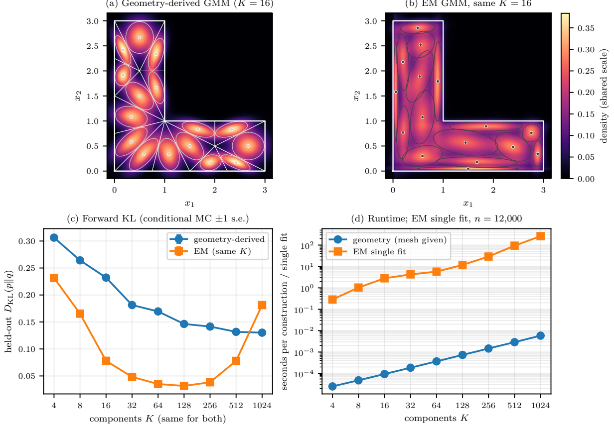
FIGURE 4. Same- K comparison of the geometry-derived GM and one fixed seeded EM fit on finite training and held-out draws. The EM held-out forward KL turns upward from K = 256 in this run. Geometry timing starts from the supplied mesh and excludes meshing; the comparison is not a global-optimality or full-benchmark claim.
