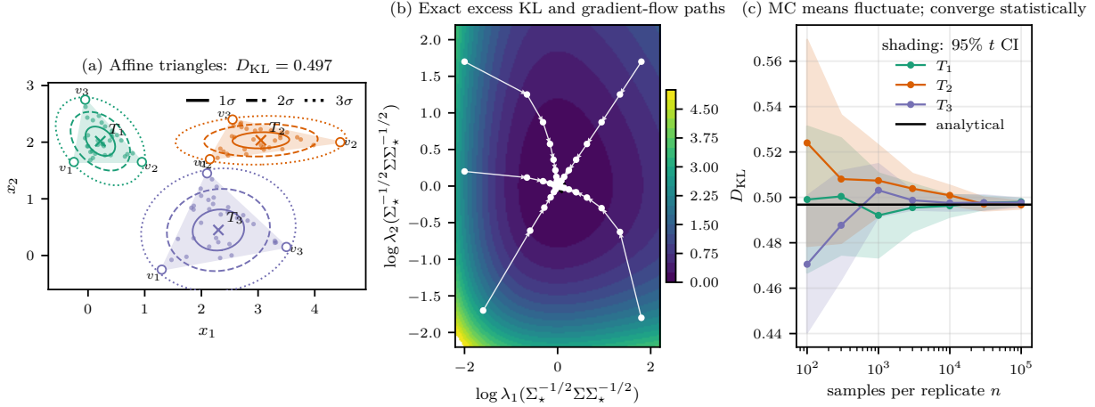
FIGURE 2. Affine triangles share the proposed analytical simplex based KL. Panel b shows the exact excess-KL landscape with gradient-flow paths; panel c shows repeated Monte Carlo estimates and 95% intervals approaching the analytical value.
