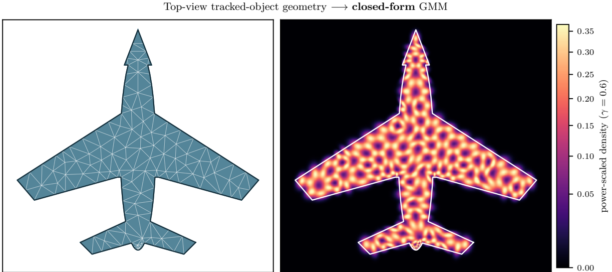
FIGURE 1. A fixed-wing planar silhouette is triangulated and directly converted into a GM, with one closed-form component per triangle.
